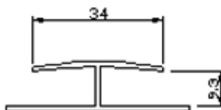
DE 680 10mm Board H-Section
