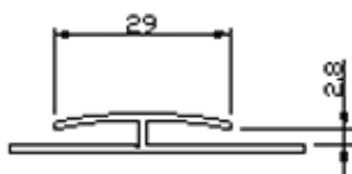
DE 695 2-3mm Board H-Section
